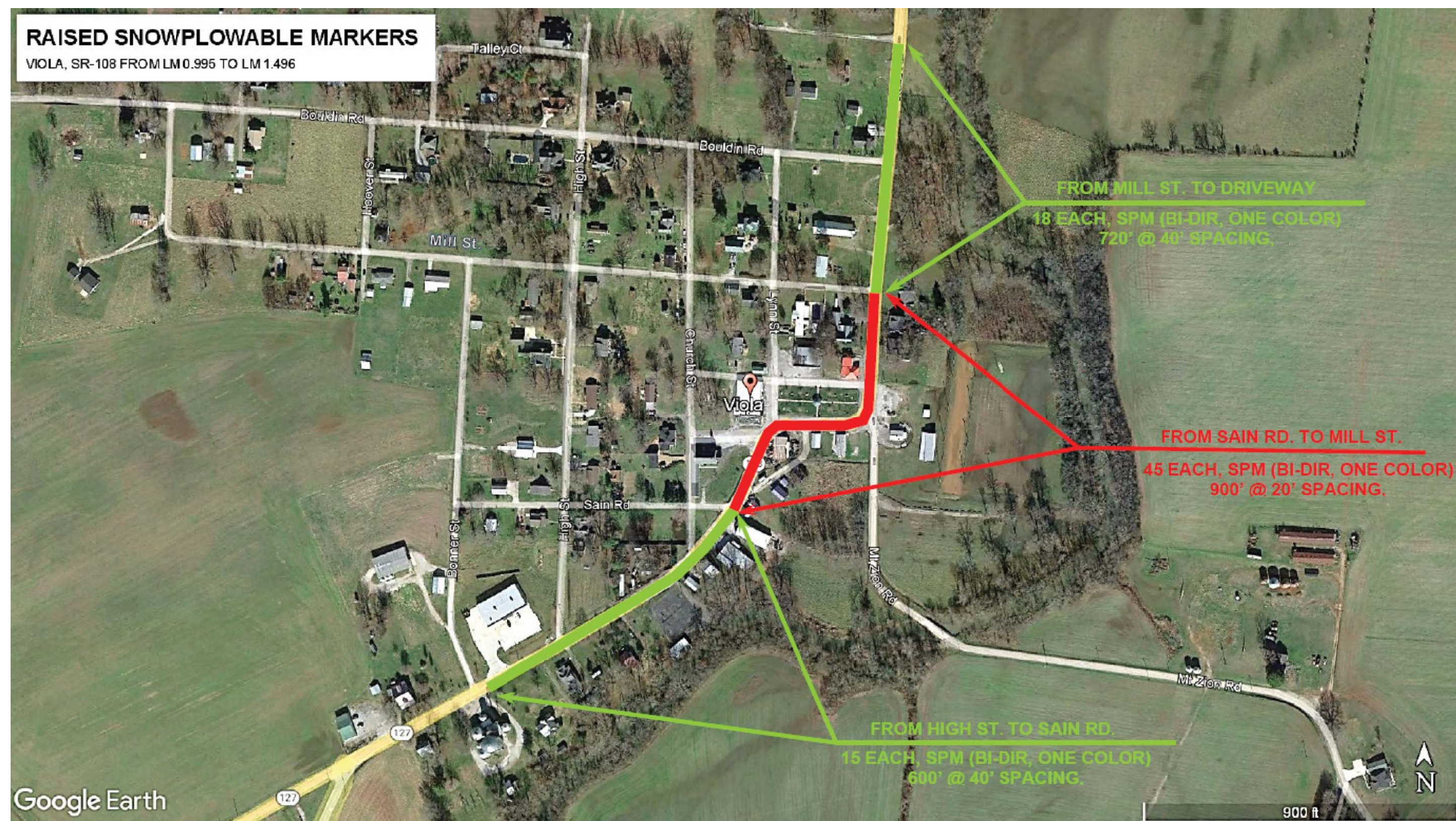
SPACING DETAIL OF RAISED SNOWPLOWABLE MARKERS ON SR-108 IN VIOLA
